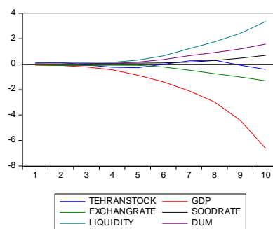
Accumulated Response of DUM to Cholesky One S.D. Innovations
