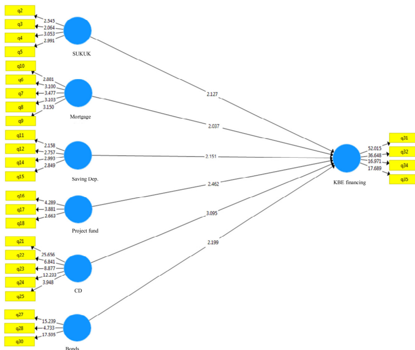
Figure 2: The Output of PLS model in standard mode
